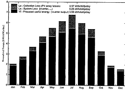
Normalized productions (per installed kWp): Nominal power 3046 kWp
