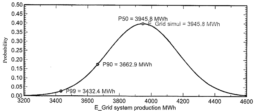
Probability distribution
