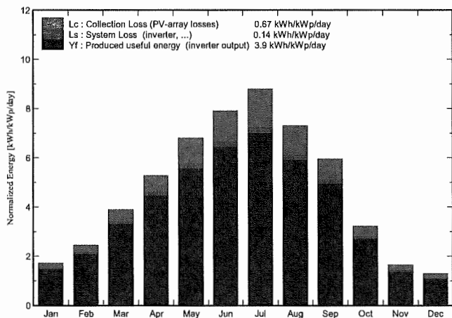
Normalized productions (per installed kWp): Nominal power 3332 kWp
