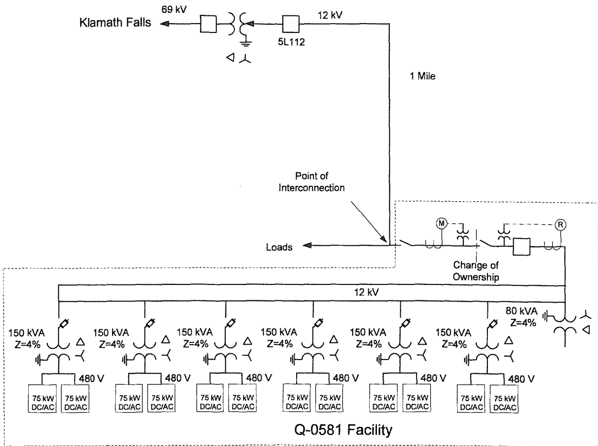
Figure 1: System One Line Diagram
