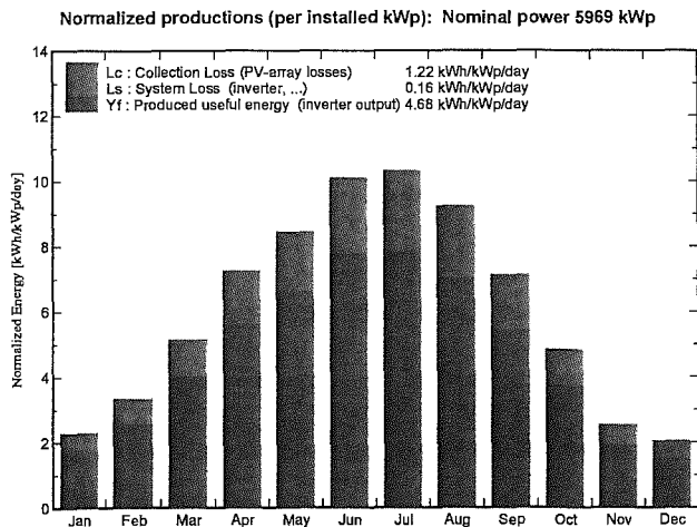
SAT0_FS395_SMA-833_r119_GCR40_NBT_5MWac Balances and main results
