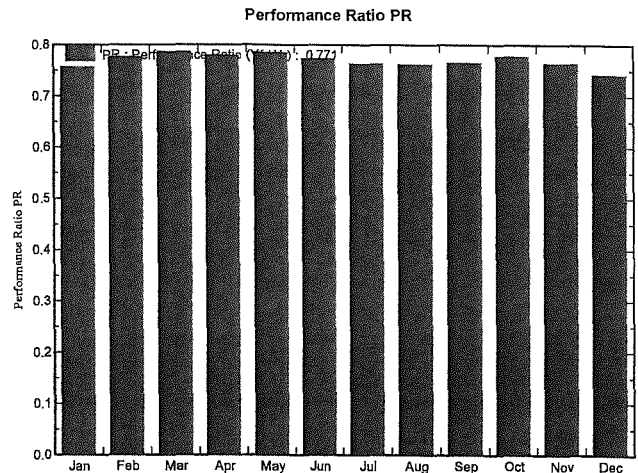
SAT0_FS395_SMA-833_r119_GCR40_NBT_5MWac Balances and main results
