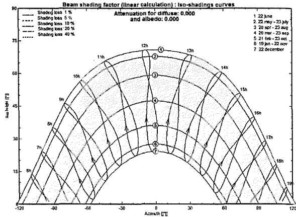
Iso-shadings diagram
