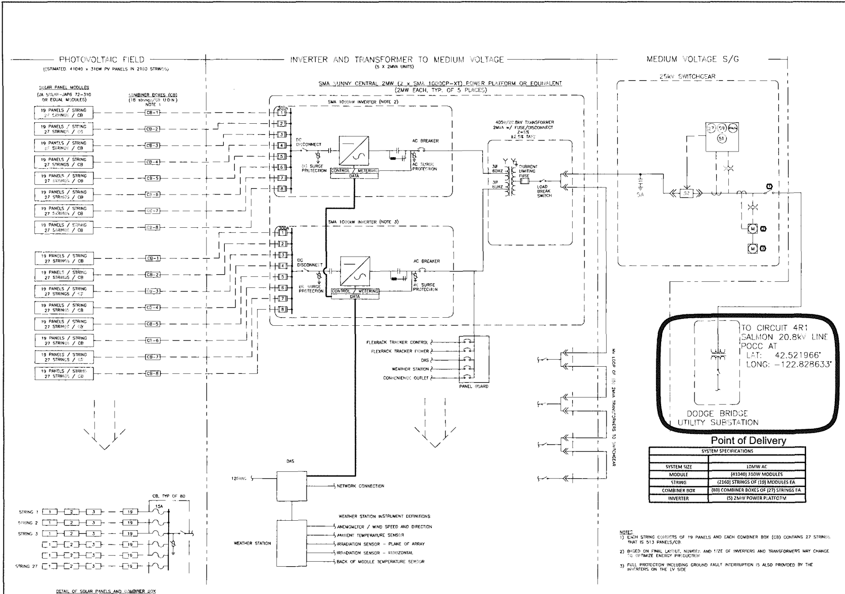
ELECTRICAL BLOCK DIAGRAM (HSAT OPTION)
