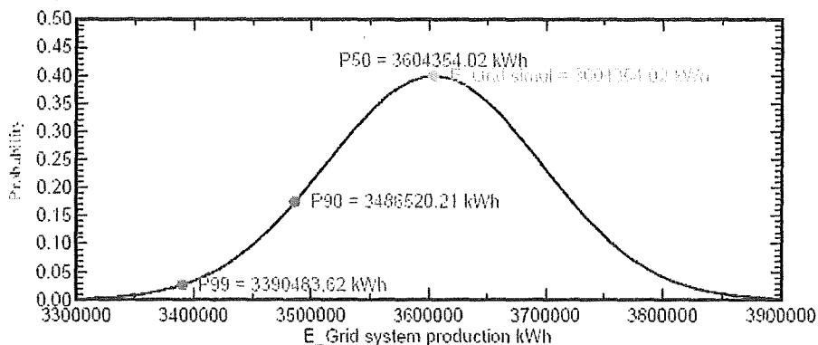
Probability distribution
