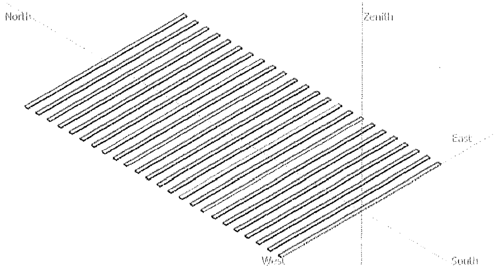
Iso-shadings diagram
