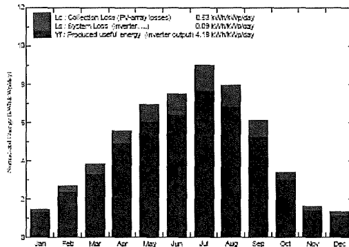
Normalized productions (per installed kWp): Nominal power 3110 kWp
