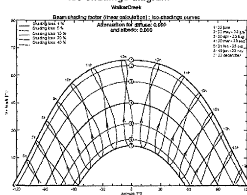
Iso-shadings diagram
