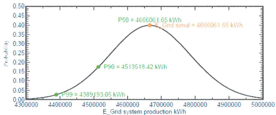
Probability distribution
