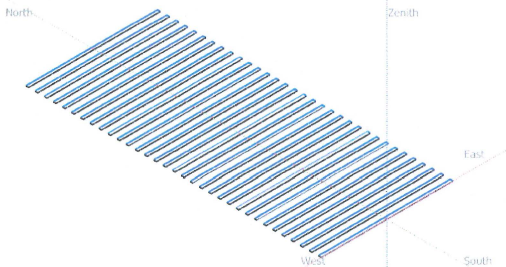
Iso-shadings diagram
