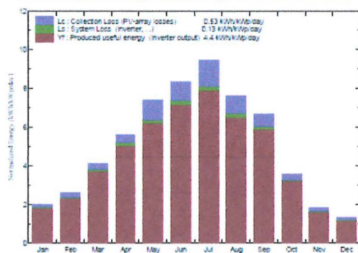
Normalized productions (per installed kWp): Nominal power 2903 kWp
