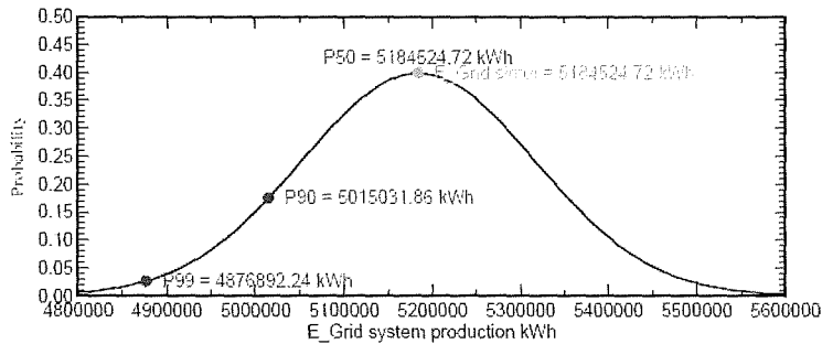
Probability distribution
