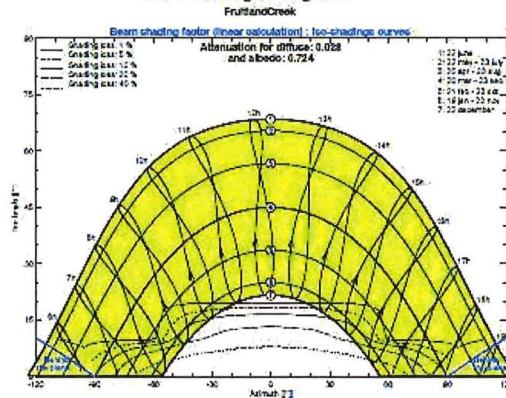
Iso-shadings diagram
