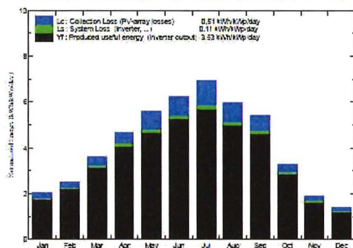
Normalized productions (per installed kWp): Nominal power 2258 kWp
