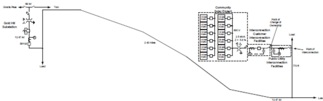
One-line Diagram Depicting the Generating Facility, Interconnection Facilities, and Metering Equipment
