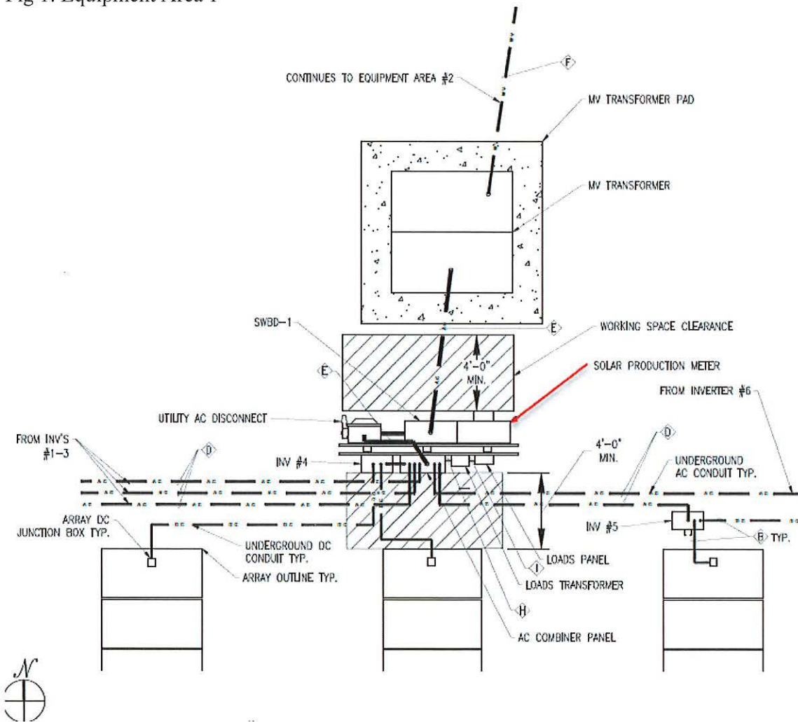
Fig 1. Equipment Area 1
