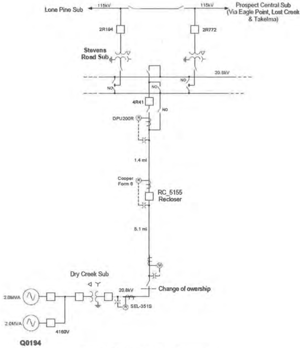
Figure 1: System One Line Diagram
