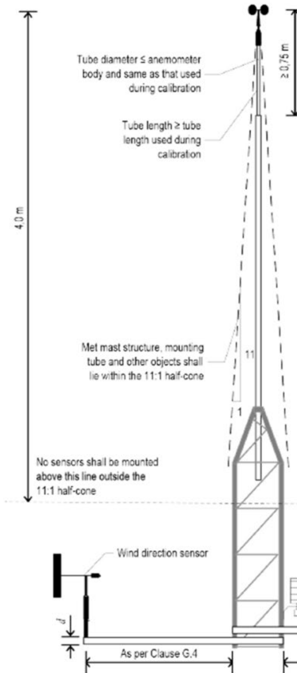
Figure G.1 – Example of a top-mounted anemometer
