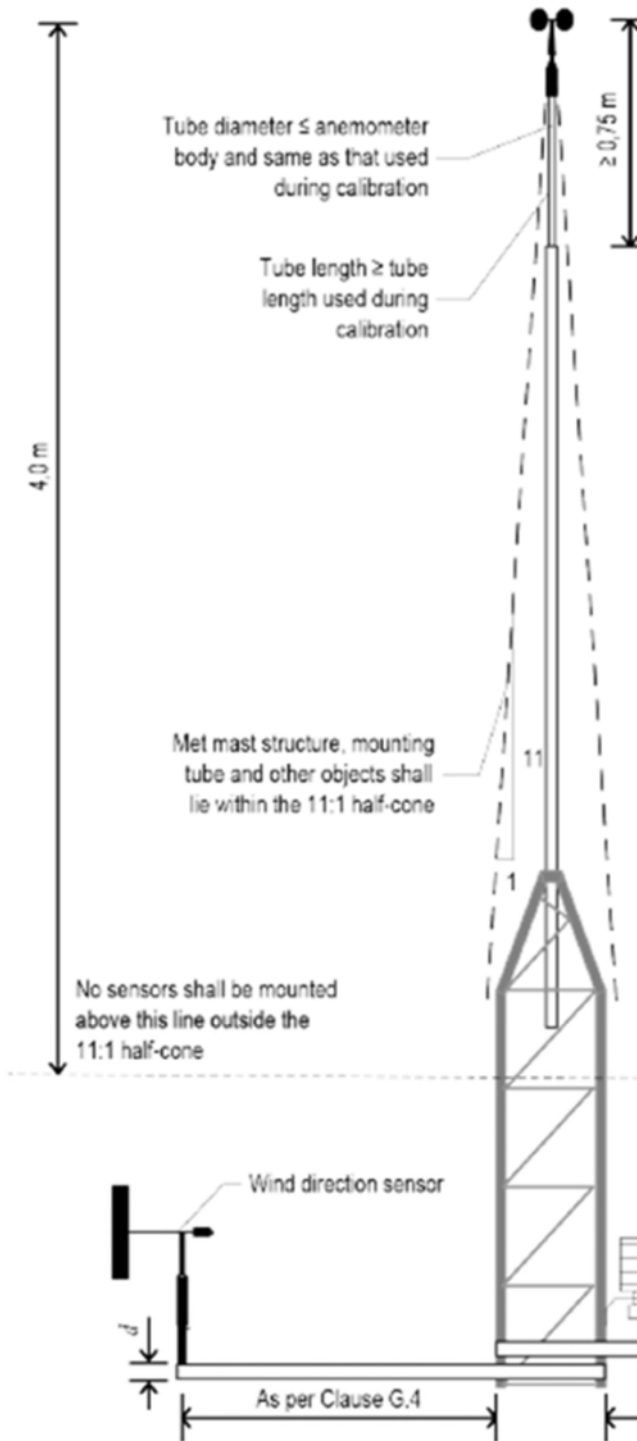
Figure G.1 – Example of a top-mounted anemor
