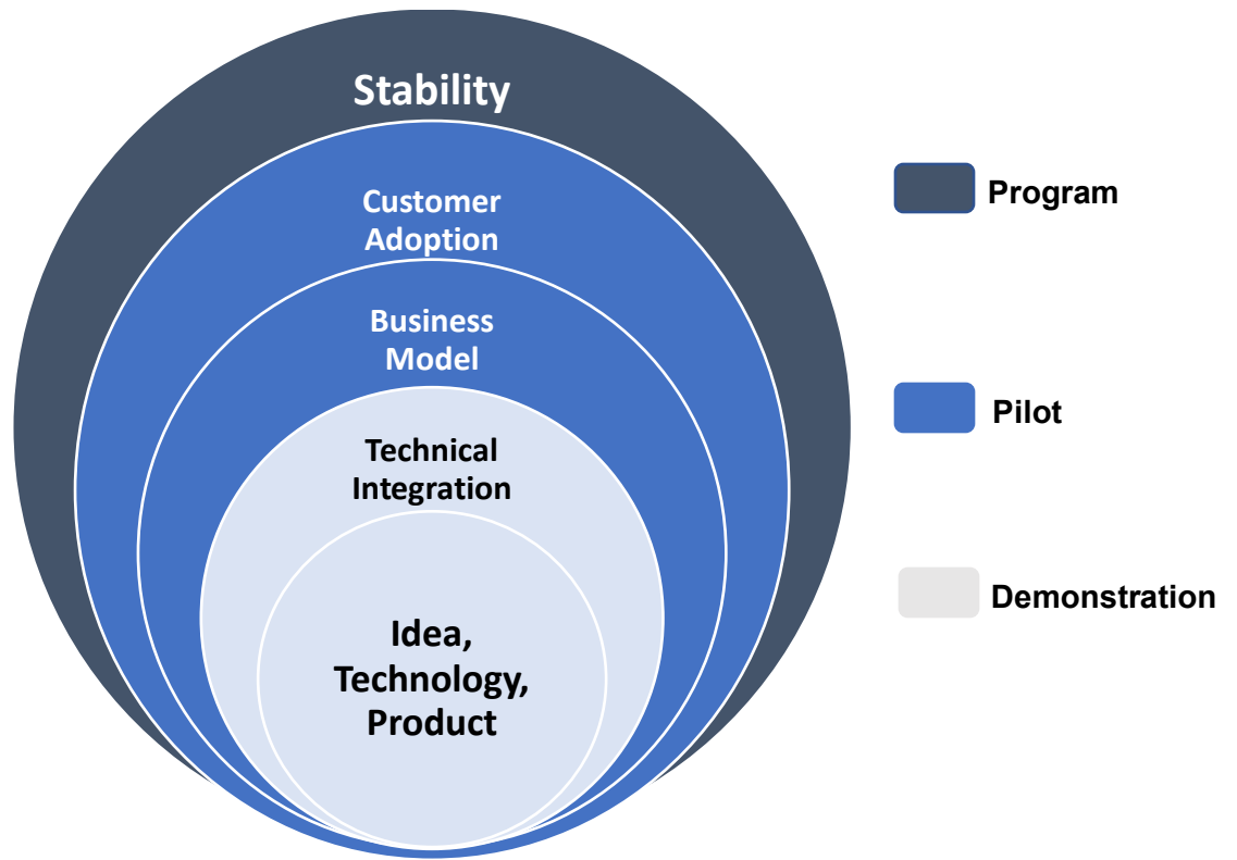
Figure 6 – Program Evolution
