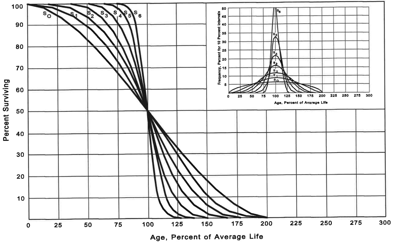
Figure 3. Symmetrical or "S" Iowa Survivor Curves
