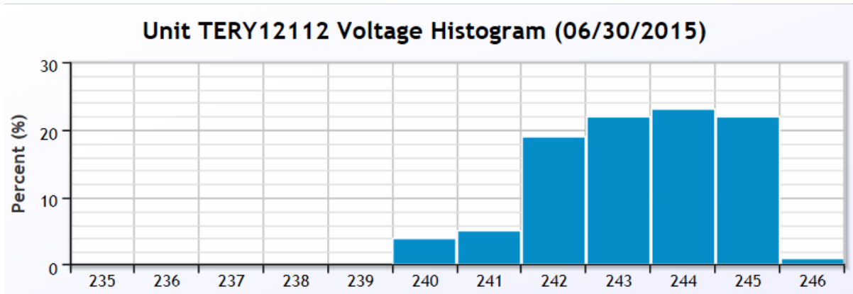
Figure 3 ENGO unit measured voltage, no VAr injection, voltage histogram
