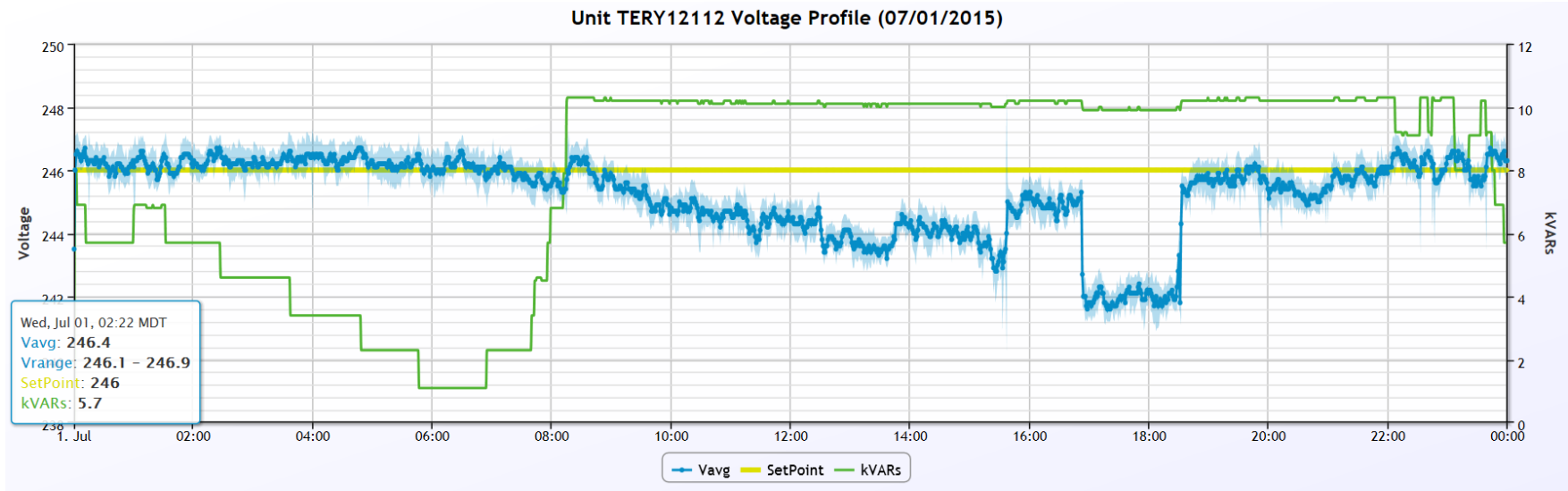
Figure 8 ENGO unit measured value, active VAr injection, voltage profile
