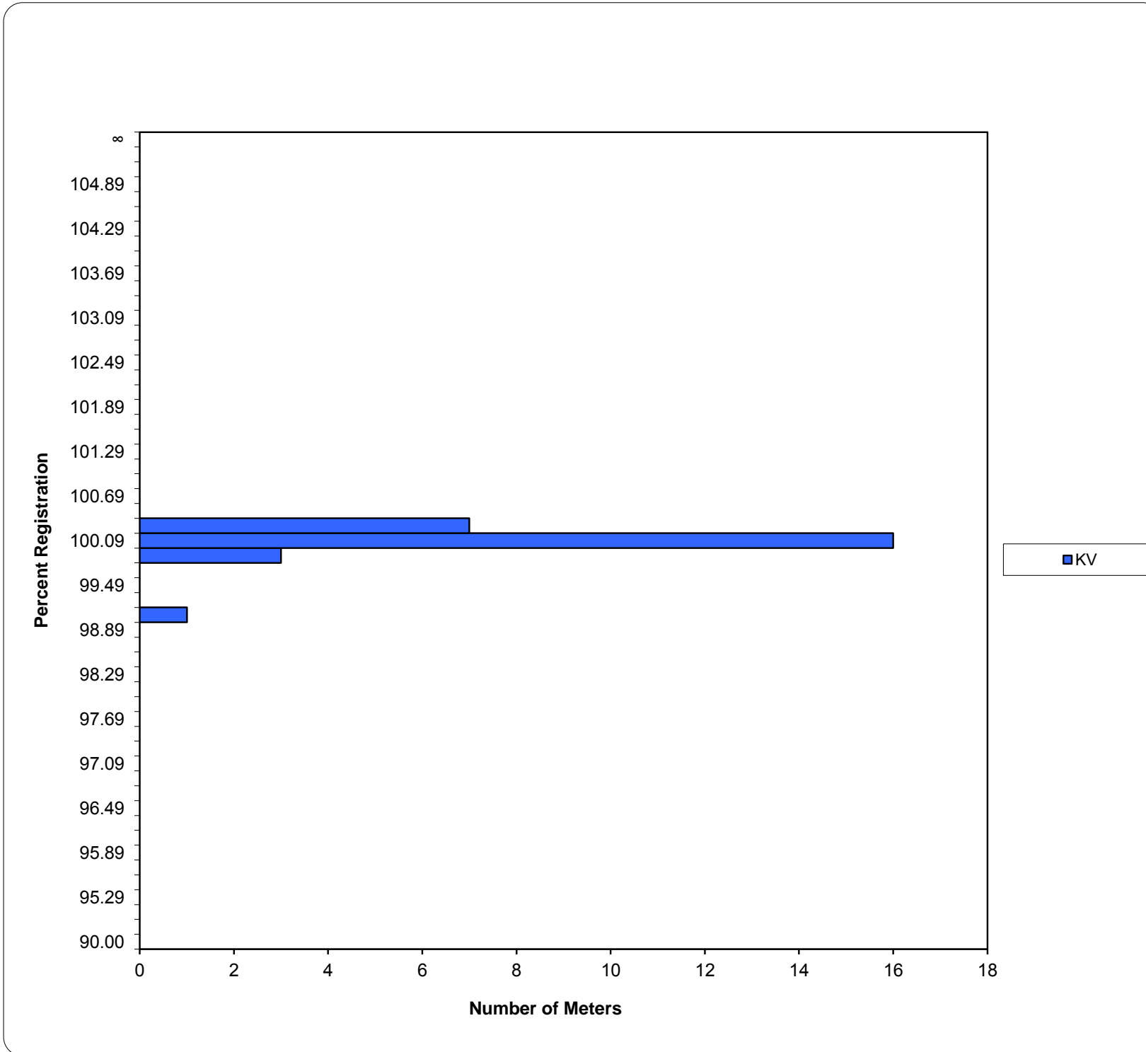
Meter Model Group: General Electric KV Weighted Avg.
