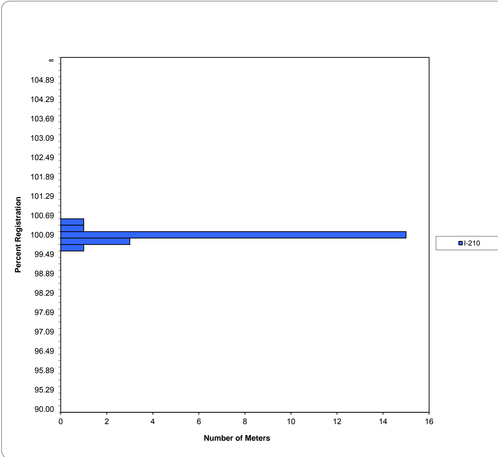
Meter Model Group: General Electric I-210 Weighted Avg.
