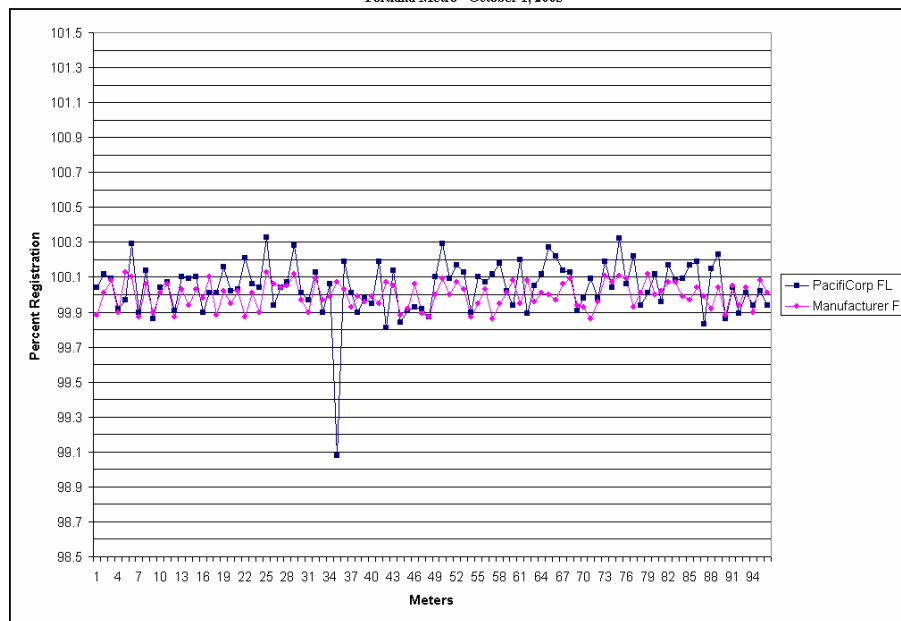
GE I-70-S Single Phase - Full Load Test - By Meter Portland Metro - October 1, 2003
