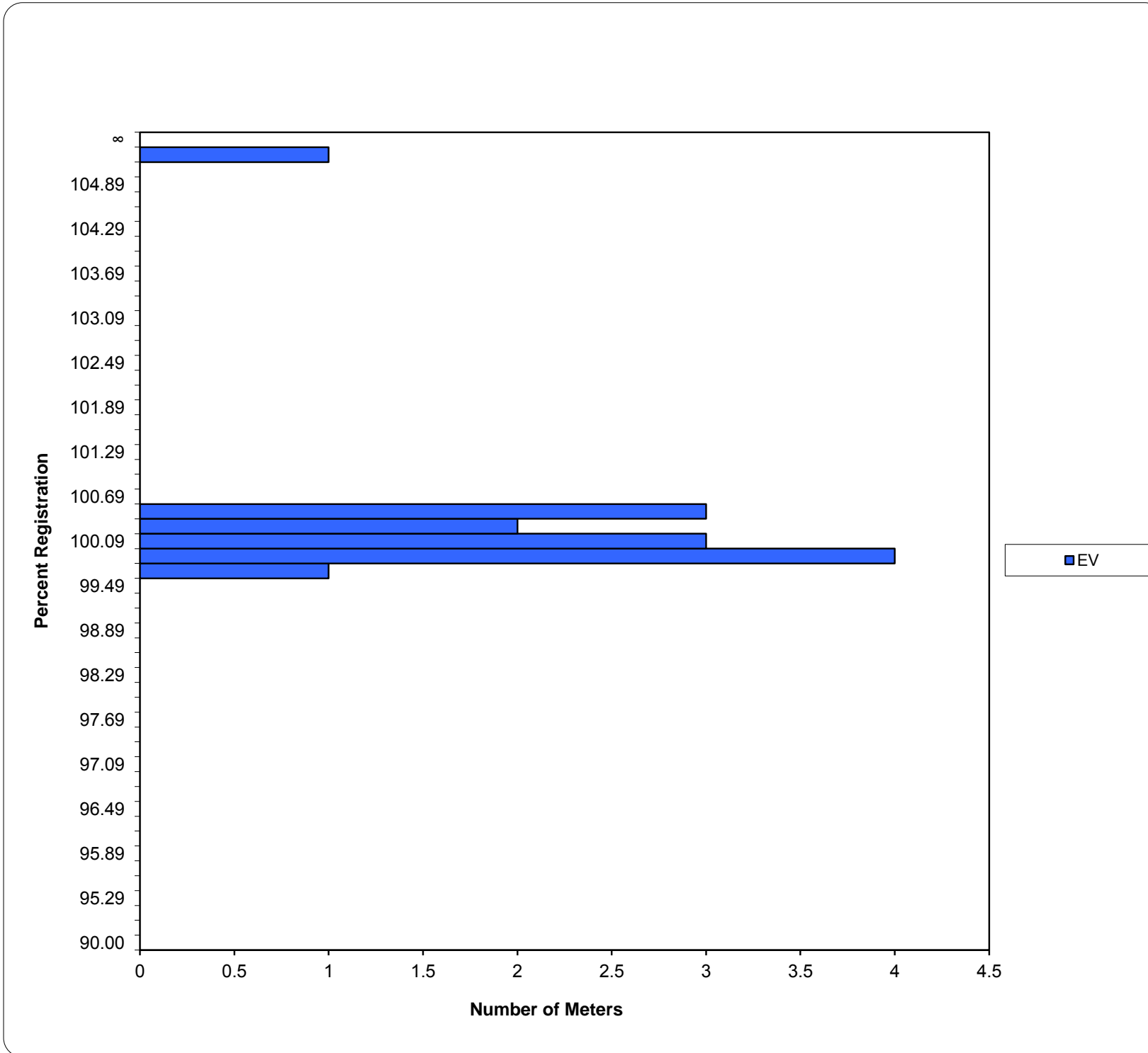
Meter Model Group: General Electric EV Weighted Avg.
