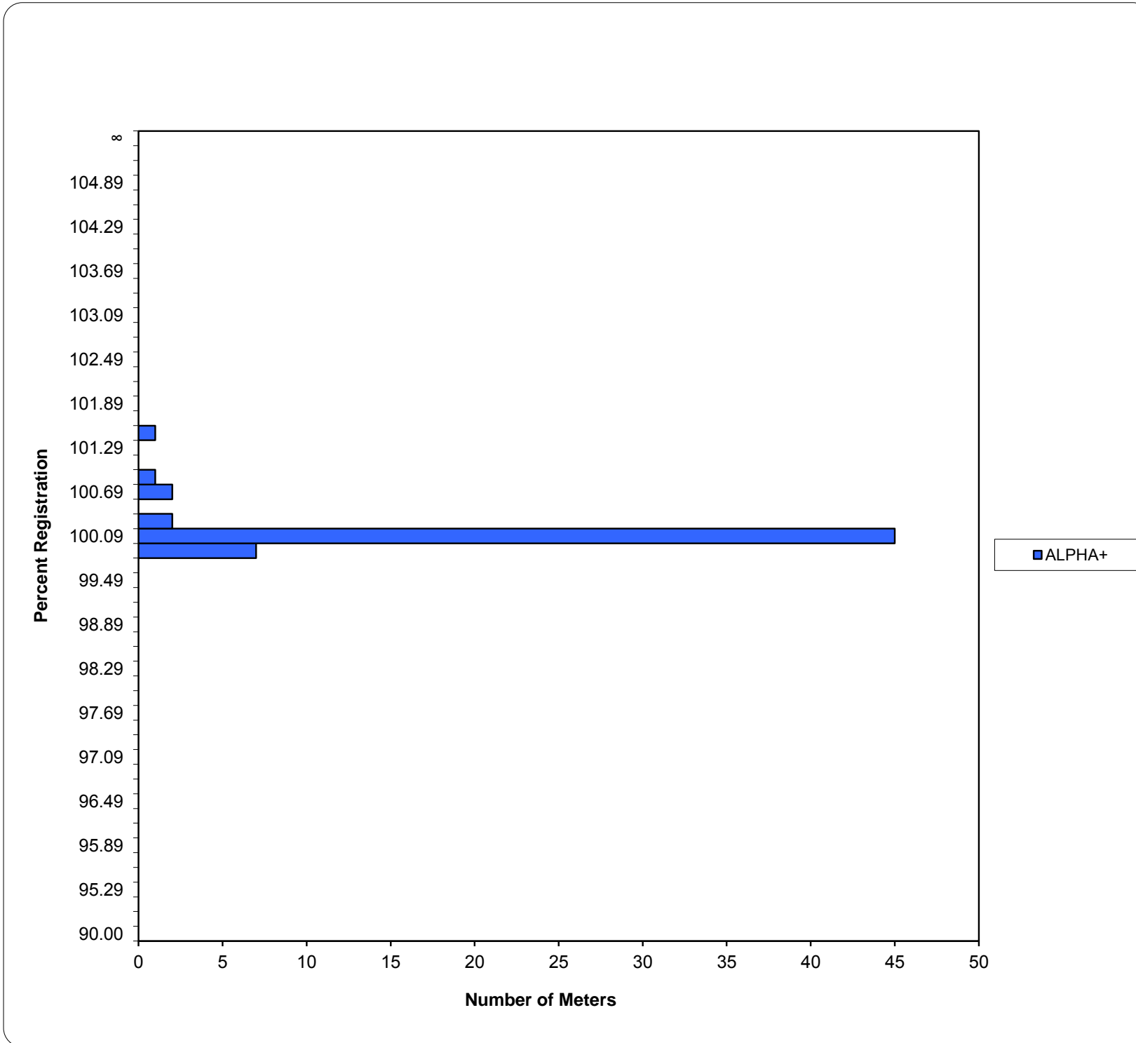
Meter Model Group: Elster ALPHA+ Weighted Avg.
