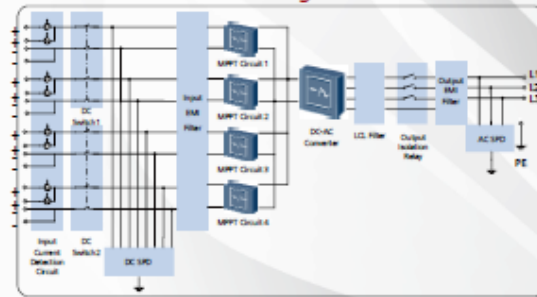
Circuit Diagram
