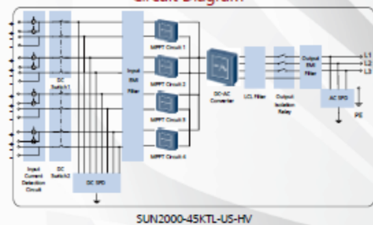
Circuit Diagram
