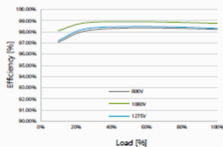
Efficiency Curve
