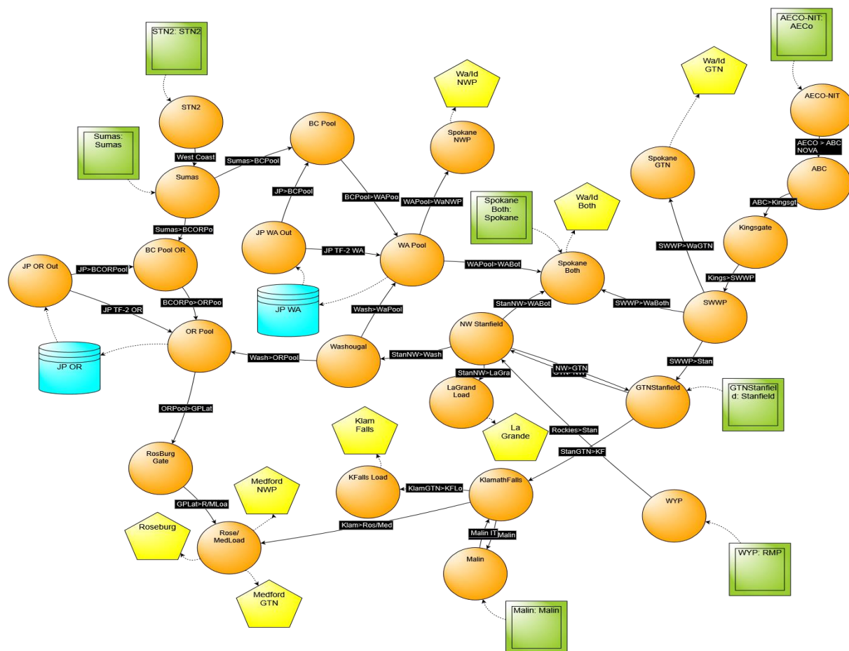
Figure 5.1 SENDOUT® Model Diagram
