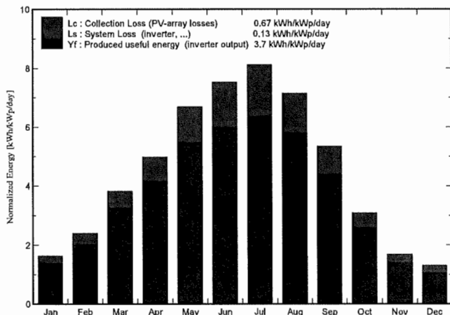
Normalized productions (per installed kWp): Nominal power 6733 kWp
