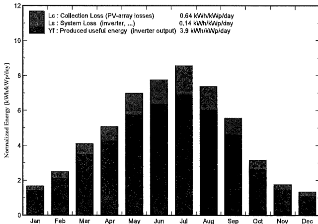
Normalized productions (per installed kWp): Nominal power 12201 kWp
