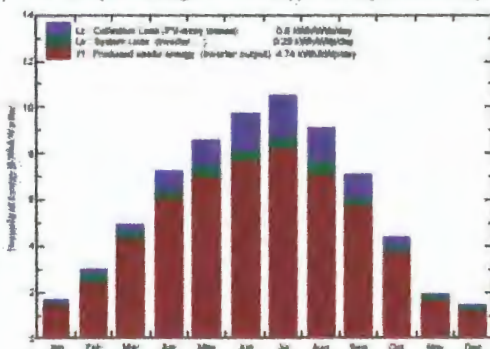
Normalized production (per installed kWp): Nominal power 12625 kWp
