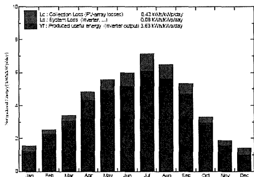
Normalized productions (per installed kWp): Nominal power 3063 kWp
