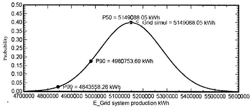
Probability distribution
