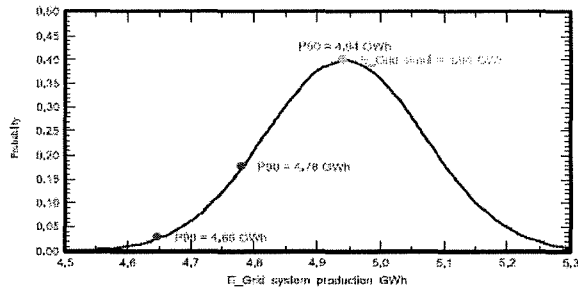
Probability distribution
