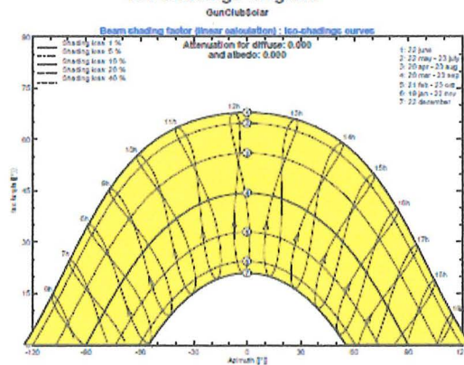
Iso-shadings diagram
