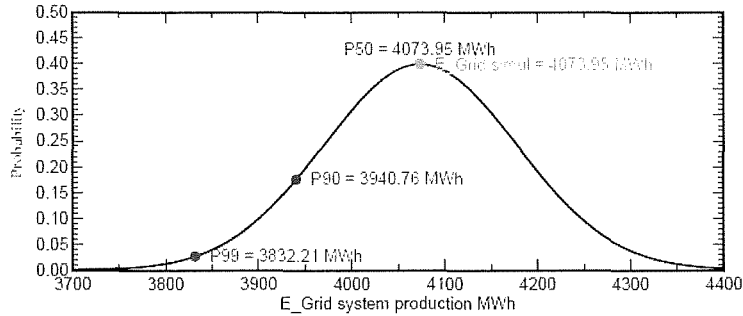
Probability distribution
