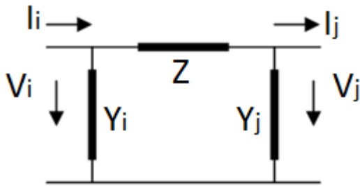
Figure 2-1 Power System Network
