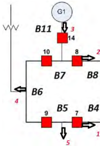
Figure 4-5 Five PMUs at a Substation
