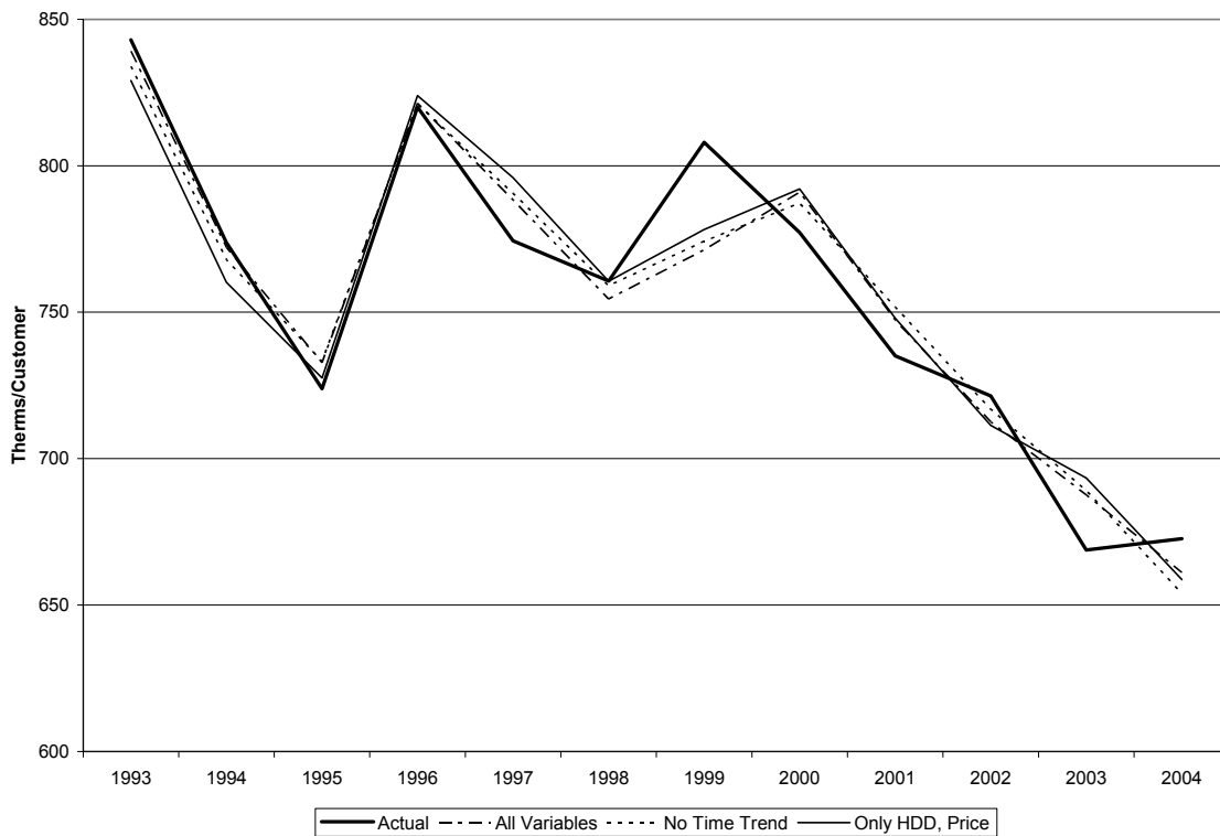
Figure 4-12: Actual versus Predicted Residential Use per Customer
